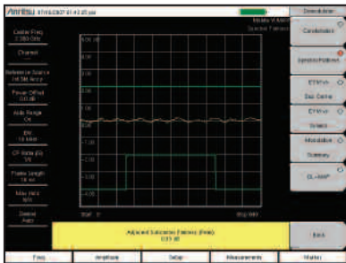
Spectral flatness uses the specified 802.16-2005 mask for pass fail analysis
