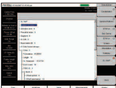
DL MAP screen displays the DL MAP zone information in a decision tree.
