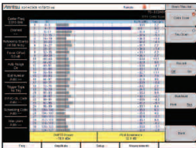
Over the Air Code Scan displays all 32 codes and its Ec/Io and Tau.
