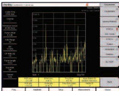
The EVM vs. Sub Carrier displays the EVM of individual subcarriers.
