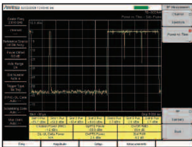
Power vs. Time screen displaying a full frame of a TD-SCDMA signal.
